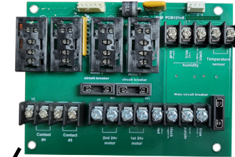
410-VCU2-24-RB Replacement Relay Board for VCU2/24, 4 relays, 4 LED lights and 3 fuse holders
