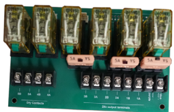
410-AEGISTEC-RB AegisTEC Relay Board, Includes PCB, 6 Relays and 3 Resettable 5A ATC Fuses
