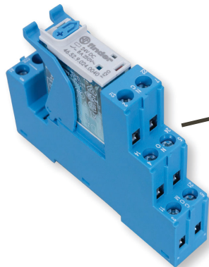
490-IMDPDT Interface Module, DPDT 8A, 24V DC, coil, LED, diode & polarity protection diode, screw terminal socket
