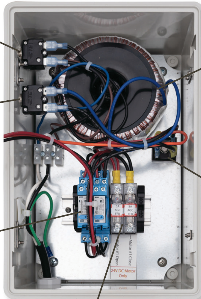
490-FFB5 Fuse, Fast Acting, Size 1/4" x 1 1/4", Glass, 5 amp, 250 VAC
